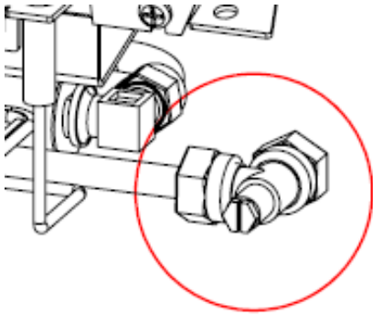
Figure 4: Bundy Pipe Fitting Location
