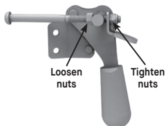
Tighten Latch
