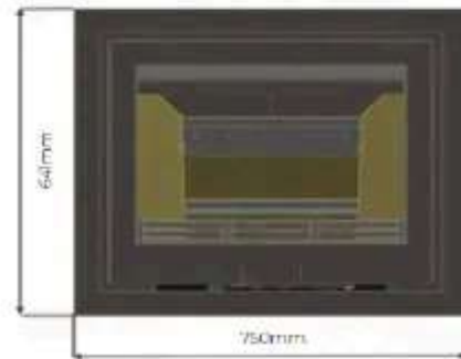
R6 & R6 SLIMLINE 4-SIDED FRAME FRONT VIEW
