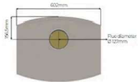
TOP VIEW FLAT SIDES
